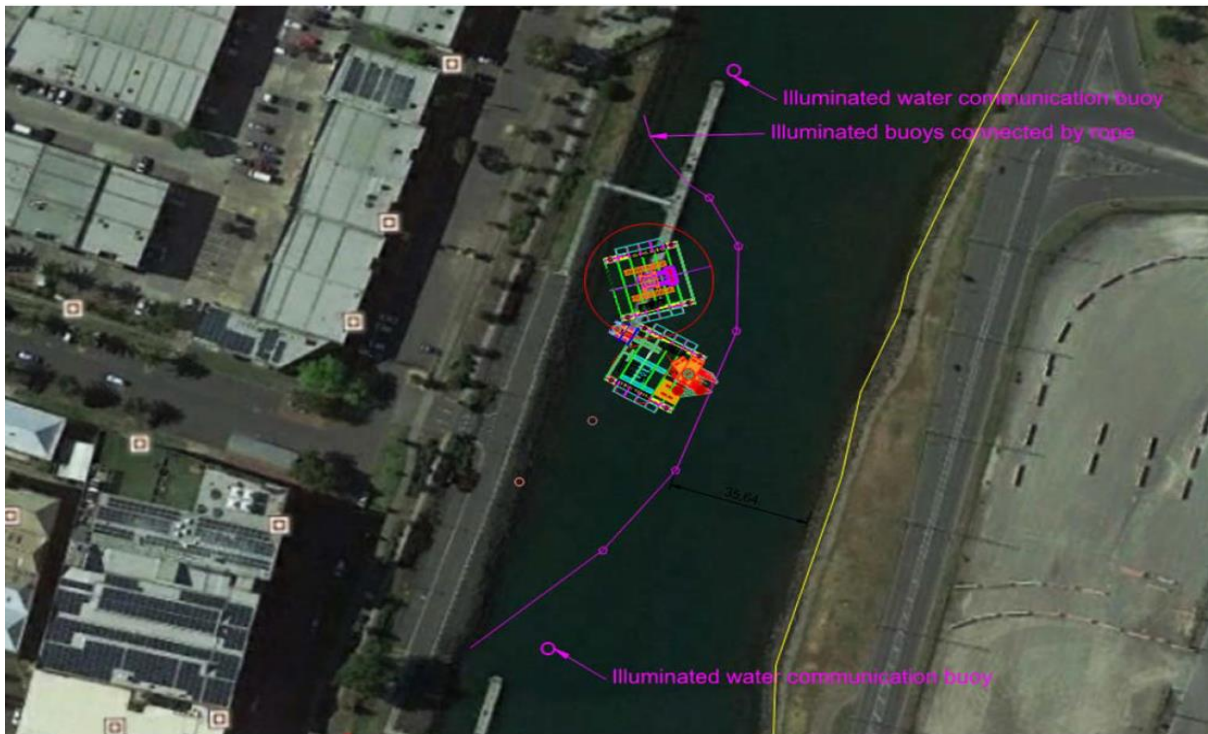
RIVER BARGE PILING SET-UP AT POSITIONS 4 & 5
